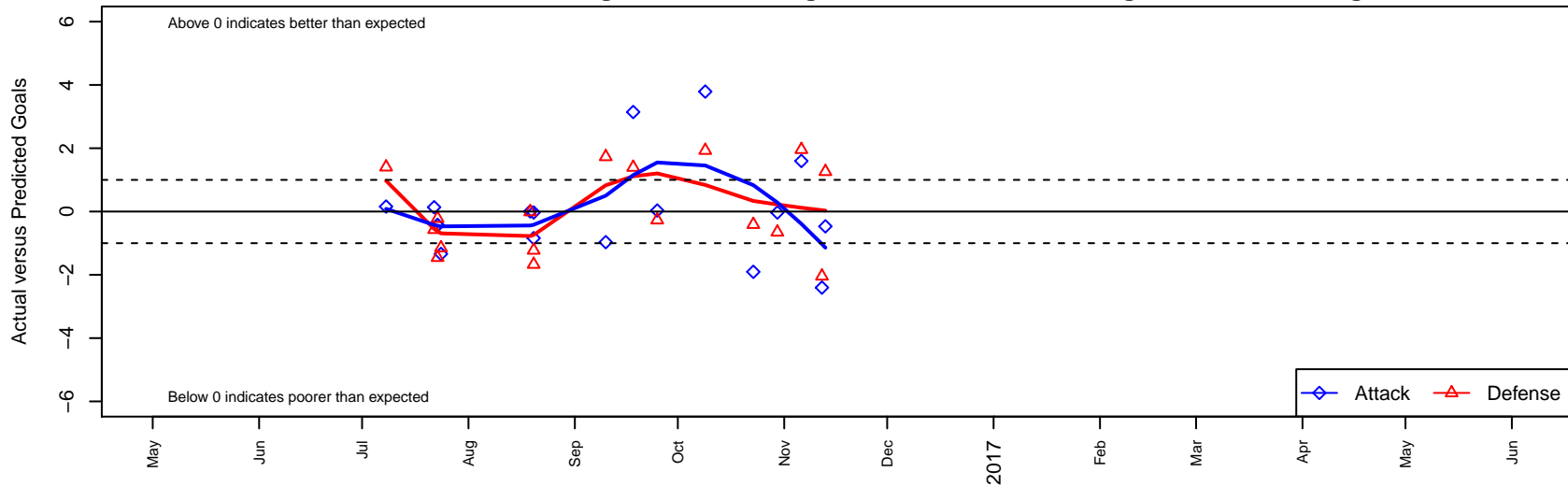
ISC Gunners Select B02 Dots are actual minus expected GF (blue circles) and GA (red triangles). Blue line is smoothed change in attack strength. Red is smoothed change in defense strength.
